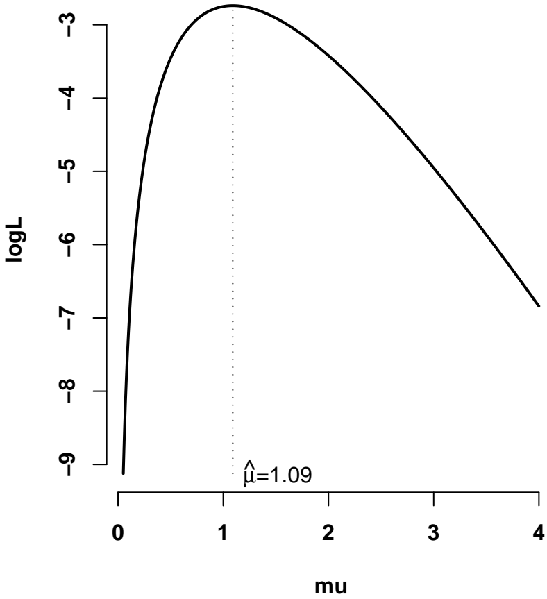
Log-likelihood for Example 5.1
